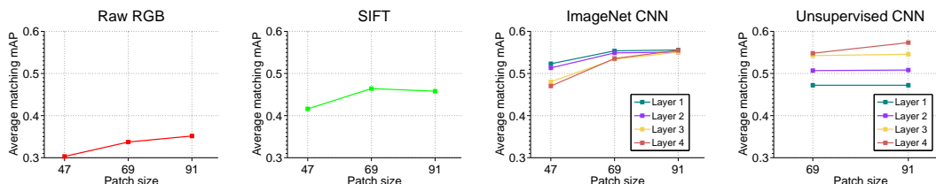
Figure 3: Parameter optimization on the larger dataset. For raw RGB and SIFT we optimized the patch size to which the detected region is normalized. For the neural nets we optimized the patch size and the network layer from which we collect the features.
