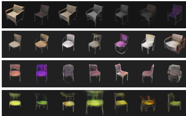
Figure 7. Images generated from single unit activations in feature maps of different fully connected layers of the 128 \times 128 network. From top to bottom: FC-1 and FC-2 of the class stream, FC-3, FC-4.
