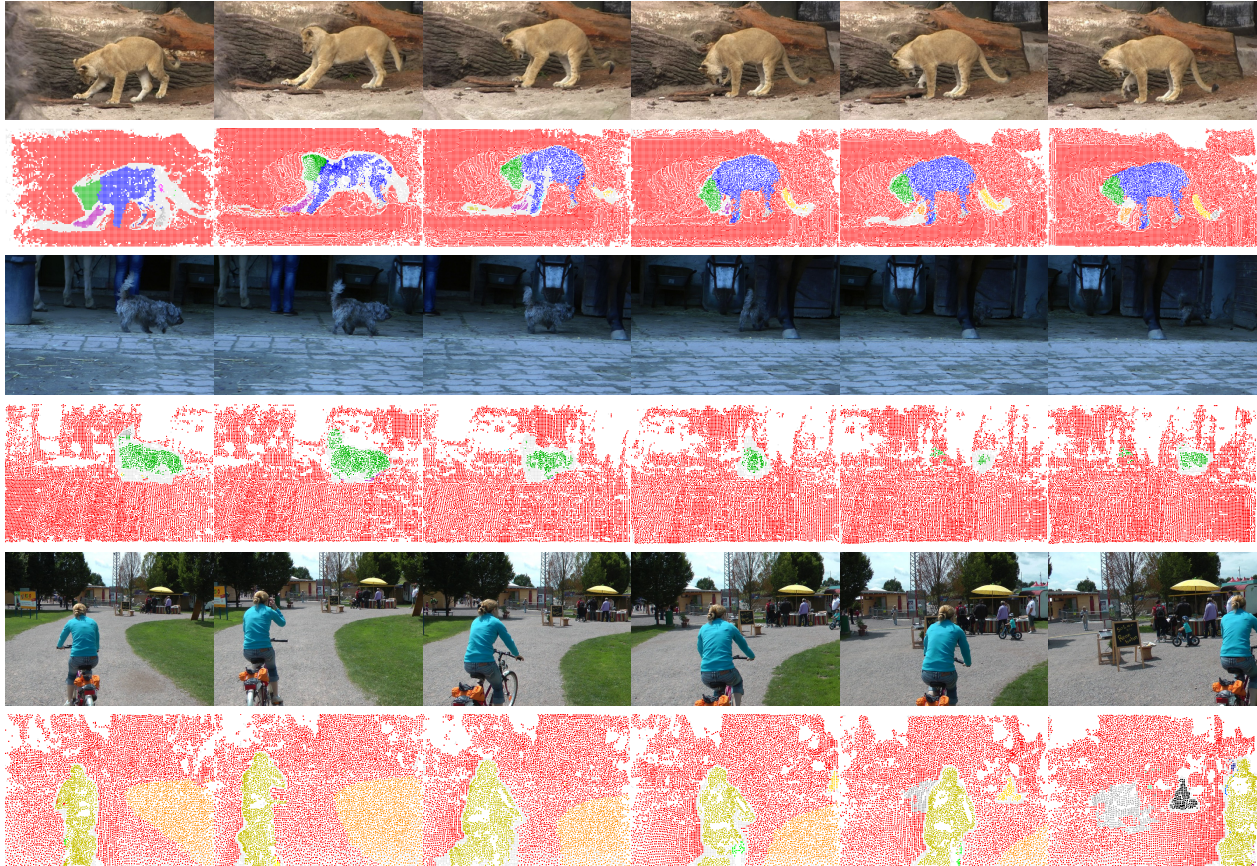
Figure 5. Frames 1, 20, 40, . . . , 100 of the lion01 sequence, frames 80, 100, . . . , 180 of the dogs01 sequence and frames 120, 140, . . . , 220 of the people05 sequence of FBMS-59 and the results of our MCe motion trajectory segmentation. Articulated motion can lead to a slight oversegmentation as in the lion01 example (top). In the dogs01 sequence (center), the dog is correctly tracked despite the occlusion. The people05 sequence (bottom row) shows the effect of a moving camera. While the moving objects in the scene (adult biker, child on the balance bike) are segmented, some static objects are segmented as well, as for example the blackboard.
