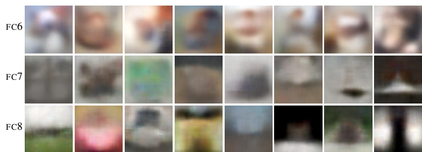
Figure 15: Reconstructions from single neuron activations in the fully connected layers of AlexNet. The FC8 neurons correspond to classes, left to right: kite, convertible, desktop computer, school bus, street sign, soup bowl, bell pepper, soccer ball.
