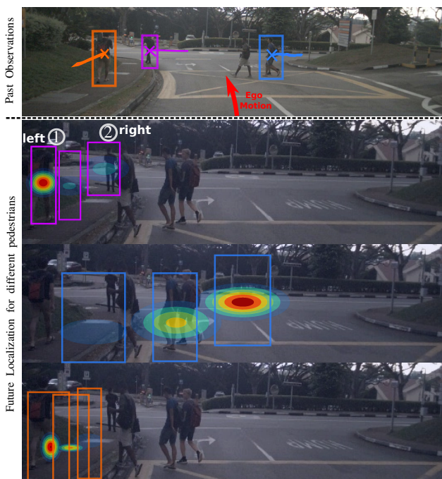
Figure 1. An example from the nuScenes dataset [9]. Given the past observations of pedestrians (colored bounding boxes (top)) and the egomotion of the car (red arrow), our framework predicts multiple modes of their future visualized by a set of bounding boxes and their distribution as an overlaid heatmap. Prediction covers possible options for (2nd row) turning left or right, (3rd row) slowing down or accelerating, (4th row) being on the sidewalk.
